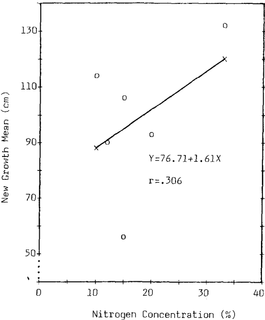
Figure 2. Effect of Nitrogen Concentration on the Growth of A. saccharum .
