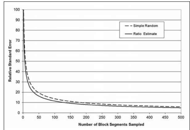
Figure 3. Comparison of relative standard error versus number of sample block segments between simple random sampling and random sampling with known block length (ratio estimate) in Syracuse, New York.
