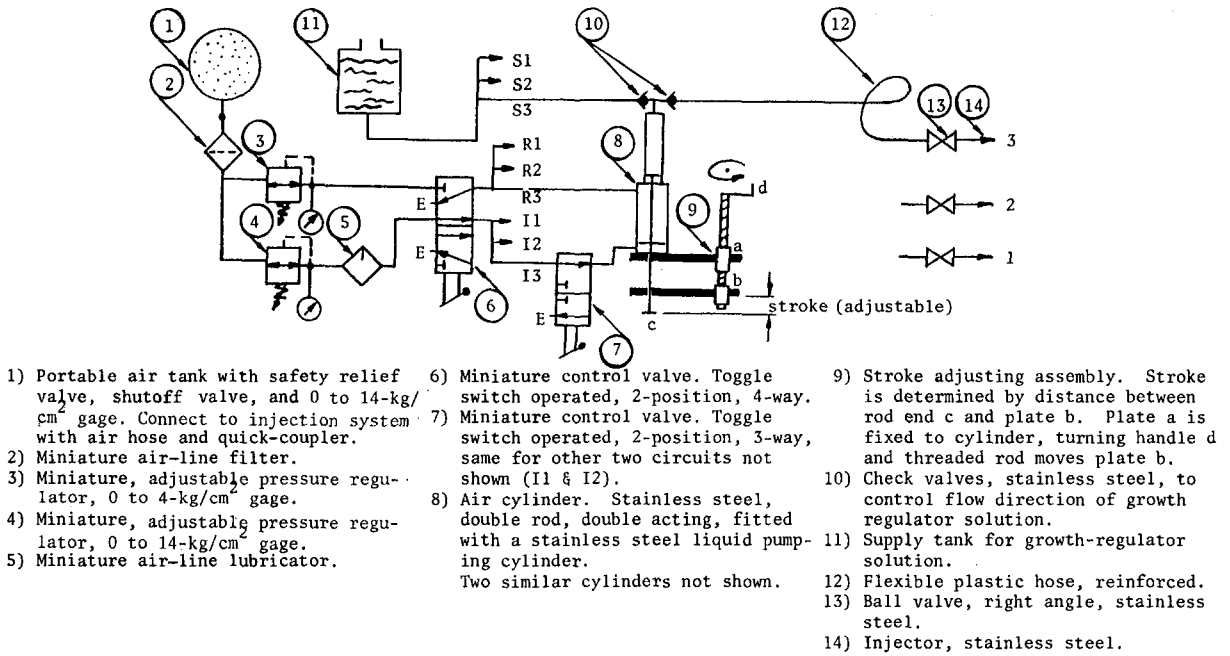
Fig. 8. Schematic details and descriptive parts list for the pneumatic and hydraulic circuits of the prototype injection equipment.
