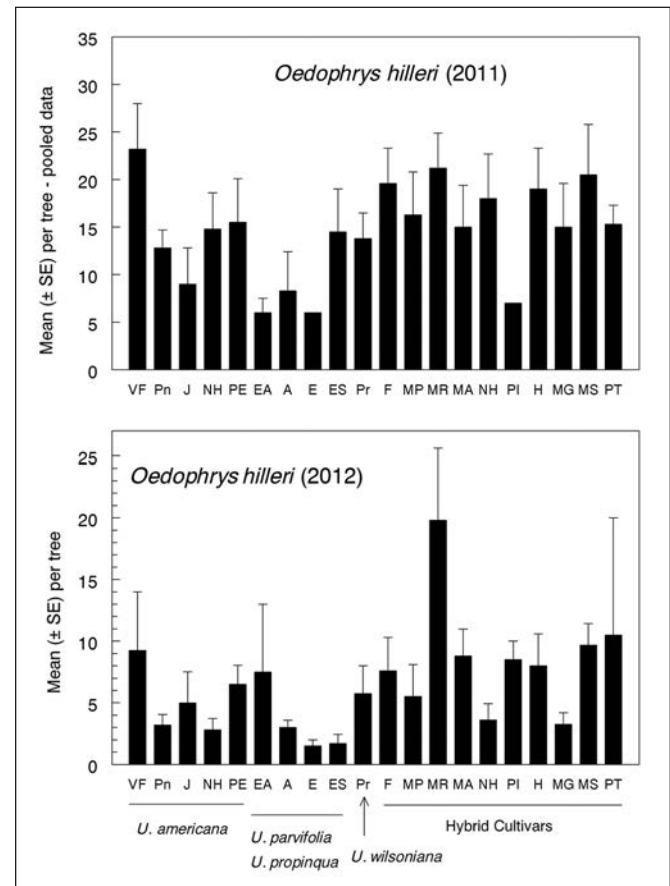
Figure 5. Leaf-notching weevil O. hilleri relative abundance on elm species and cultivars. Cultivar differences were significant each year ( F_{19,59} = 2.54, P < 0.01 in 2011; F_{19,52} = 2.04, P < 0.05 in 2012). Elms with Asian parentage as a group had fewer weevils than either American or hybrid cultivars in 2011 and fewer than hybrids in 2012 (linear contrasts, P < 0.01 ).
