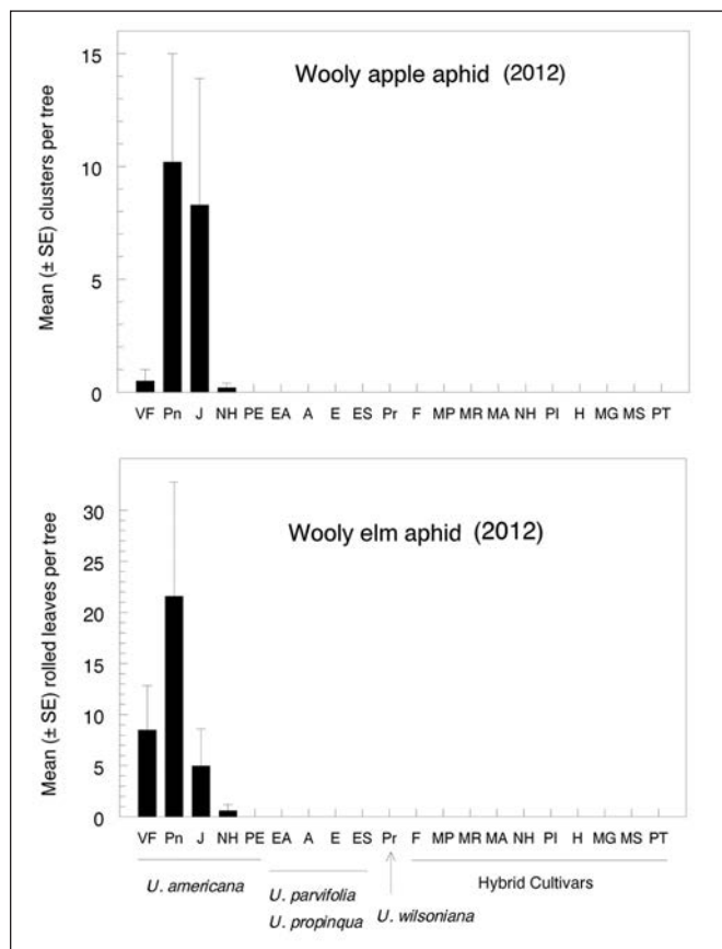
Figure 6. Rolled leaves with woolly elm aphids and rosettes of deformed leaves caused by feeding of woolly apple aphids were restricted to U. americana . Within American elms, there were significant cultivar differences in susceptibility to each pest (Kruskal-Wallis, P \leq 0.05 ).
