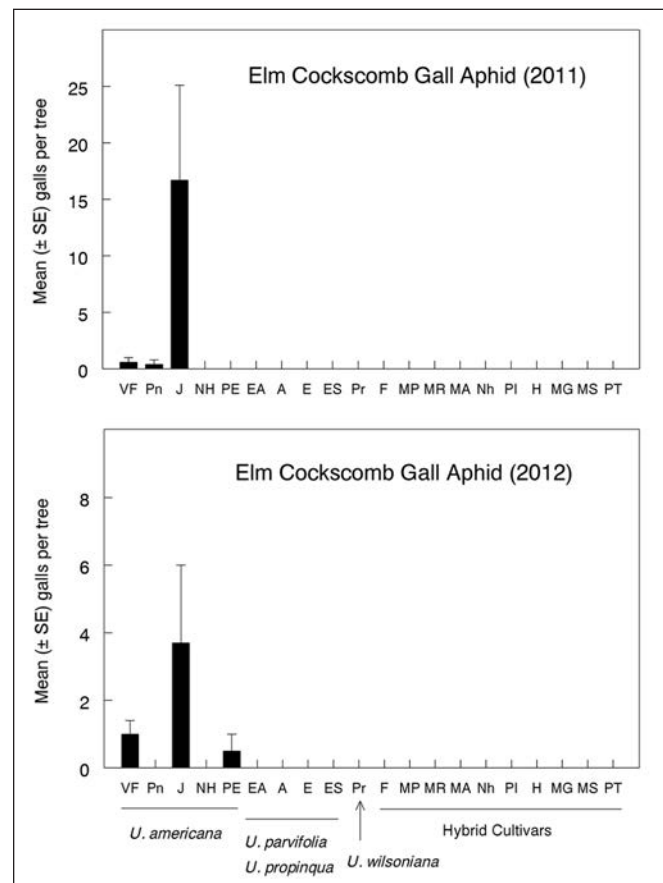
Figure 7. Elm cockscomb gall aphid was only found on American elms, among which its abundance differed each year (Kruskal-Wallis, P < 0.001 ).
