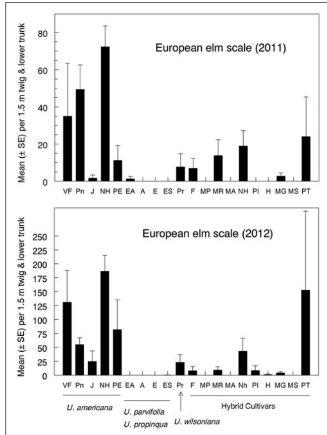
Figure 3. European elm scale relative abundance on elm species and cultivars. There were significant differences among cultivars in each year (Kruskal-Wallis, P < 0.001 ).
