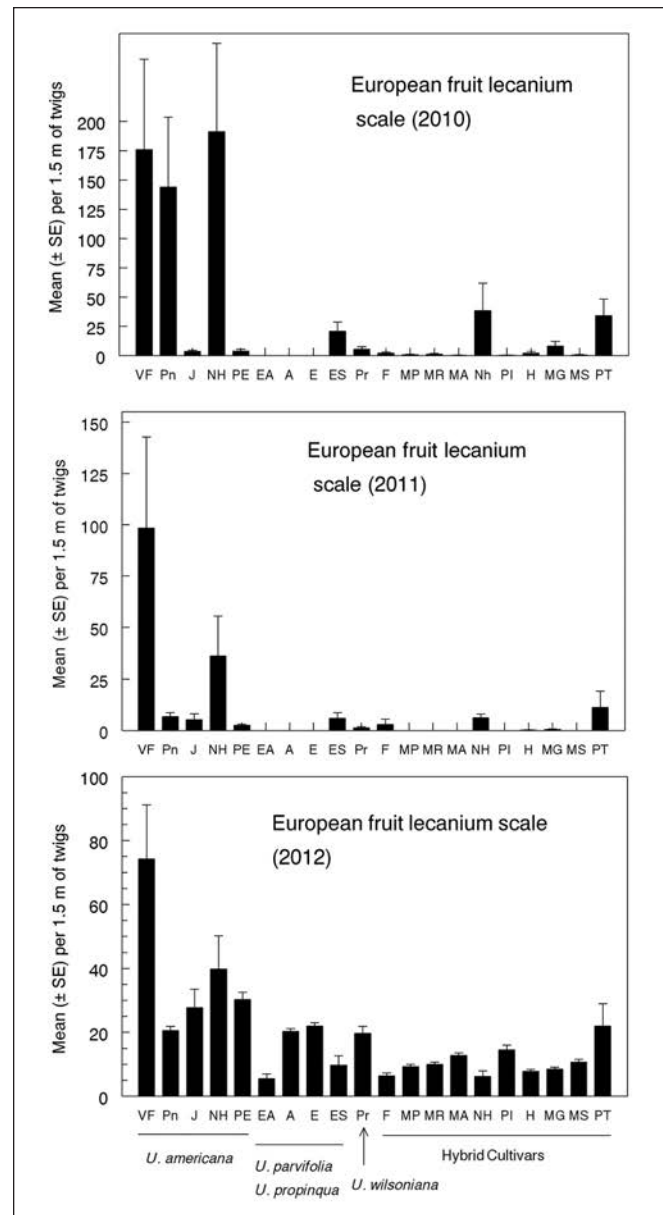
Figure 2. European fruit lecanium relative abundance on elm species and cultivars. Cultivars abbreviations are indicated in Table 1. There were significant cultivars differences each year (Kruskal-Wallis, P < 0.001 ). Absence of variance (means of zero) for some cultivars precluded parametric analyses in 2010–11. U. americana cultivars as a group were more heavily infested than those having Asian parentage ( U. parvifolia + propinqua + wilsoniana ), or hybrid cultivars in 2012 (ANOVA, linear contrasts, P < 0.01 ).
