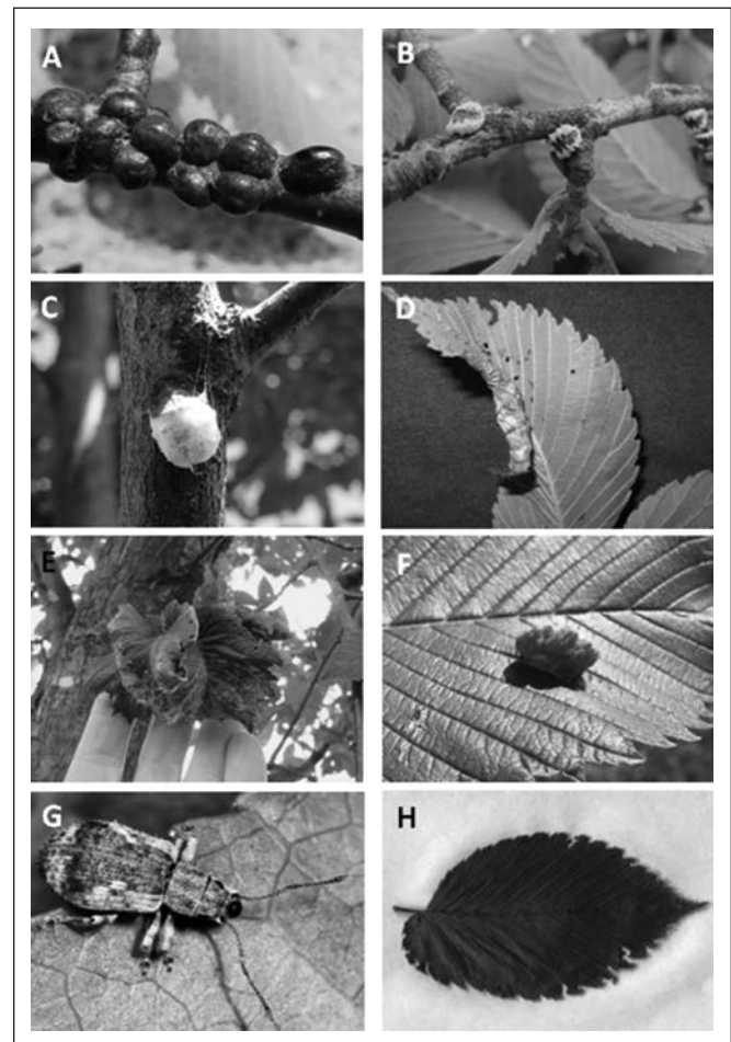
Figure 1. Insect pests and damage symptoms evaluated in the Kentucky portion of the National Elm Trial from 2010–2012: (A) European fruit lecanium ( Parthenolecanium corni ), (B) European elm scale ( Eriococcus spuria ), (C) cottony maple scale ( Pulvinaria innumerabilis ), (D) woolly elm aphid ( Eriosoma americanum ), (E) woolly apple aphid ( Eriosoma lanigerum ), (F) elm cockscomb gall aphid ( Colopha ulmicola ), (G) Oedophrys hilleri weevil (photo by S. Cresswell), (H) leaf notching by O. hilleri . See Condra et al. (2010) for images of previously evaluated pests.
