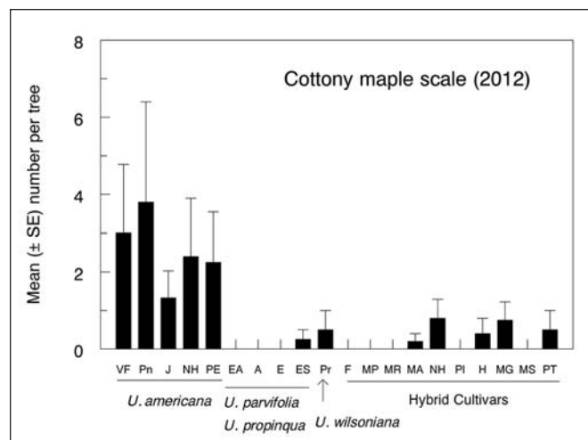
Figure 4. Cottony maple scale whole-tree counts in 2012, the first year it was noted on some trees. Low numbers, high variance, and reduced replication due to loss of some trees contributed to no detectable cultivar differences (Kruskal-Wallis, P = 0.48 ).
