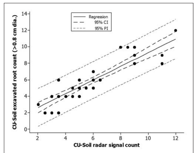
Figure 4. Regression output showing confidence and prediction intervals for a relationship in CU-Structural Soil comparing ground-penetrating radar output to excavated actual root counts (N = 40 measurement sections, not all data points visible due to overlap). Relationship shown: excavated root count = 0.97 + 0.83 radar signal count; r^2 = 0.81 .
