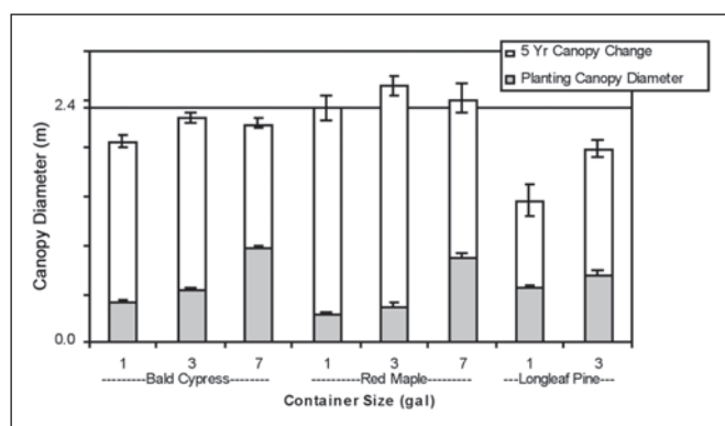
Figure 2. Canopy diameter (mean ± SE) of baldcypress, red maple and longleaf pine trees in #1, #3, and #7 container sizes at time of initial planting and five years later. Shaded base is canopy diameter at time of planting, nonshaded top section reflects five-year change in canopy diameter; bar total represents cumulative five-year canopy diameter. Reference value shown of 2.4 m represents the canopy diameter required to achieve theoretical 50% cover assuming 100% survival and an initial tree planting density of 174/ha.
