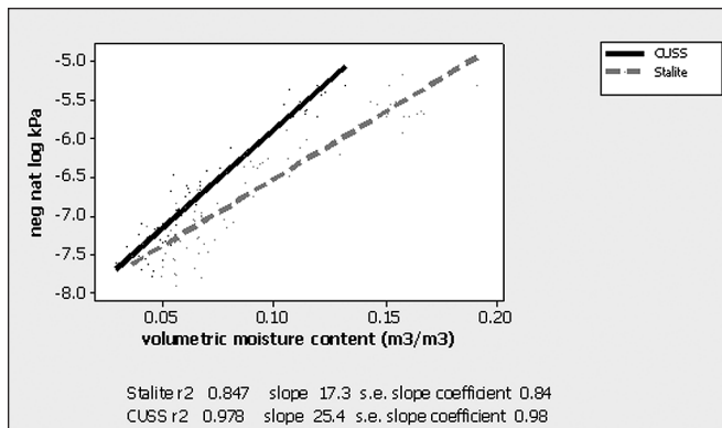
Figure 2. Predawn leaf water potential data transformed into a negative natural log and plotted for linear regression slope analysis for treatment comparison and assignment of high matric potential (assigned at 1500 kPa or -7.31 to determine plant available moisture endpoint). Regression line endpoints correspond with minimum and maximum value observations on the x axis for each treatment.
