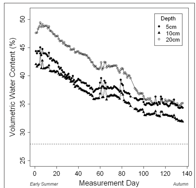
Figure 4. Soil volumetric water content at three depths beneath pervious pavement. Each data point represents the mean value of five probes (in five replicate plots). The dotted line represents the field capacity of the soil.
