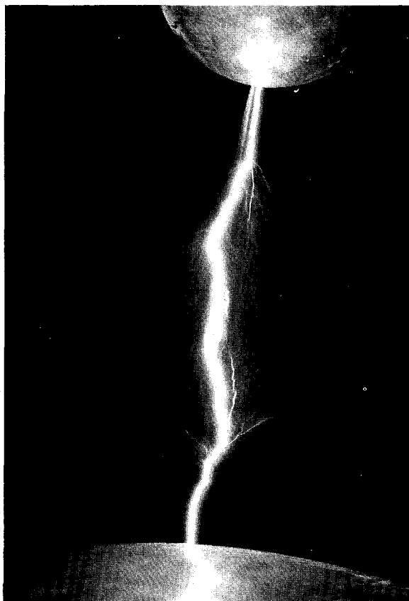
Figure 3. A D- stroke. The spark starts at the smaller top electrode which would be the cloud. Before the spark propagates all the way to the ground on the larger electrode, it is met by a return stroke.
