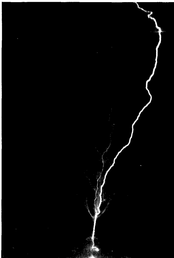
Figure 2. A U+ stroke. The spark starts at the bottom smaller electrode and propagates upward to the larger electrode which acts as the negatively charged cloud. Note branching in direction of propagation.
