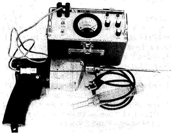
Figure 2. Field ohmmeter and electrode accessories for measurement of internal discoloration and decay and for measurements of the cambial zone.
