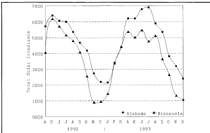
Fig. 1. Monthly average total solar radiation (K↓) in Winton, Minnesota and Auburn, Alabama for 1992 and 1993. Units for irradiance from integrated measurements = Wh m -2 .
