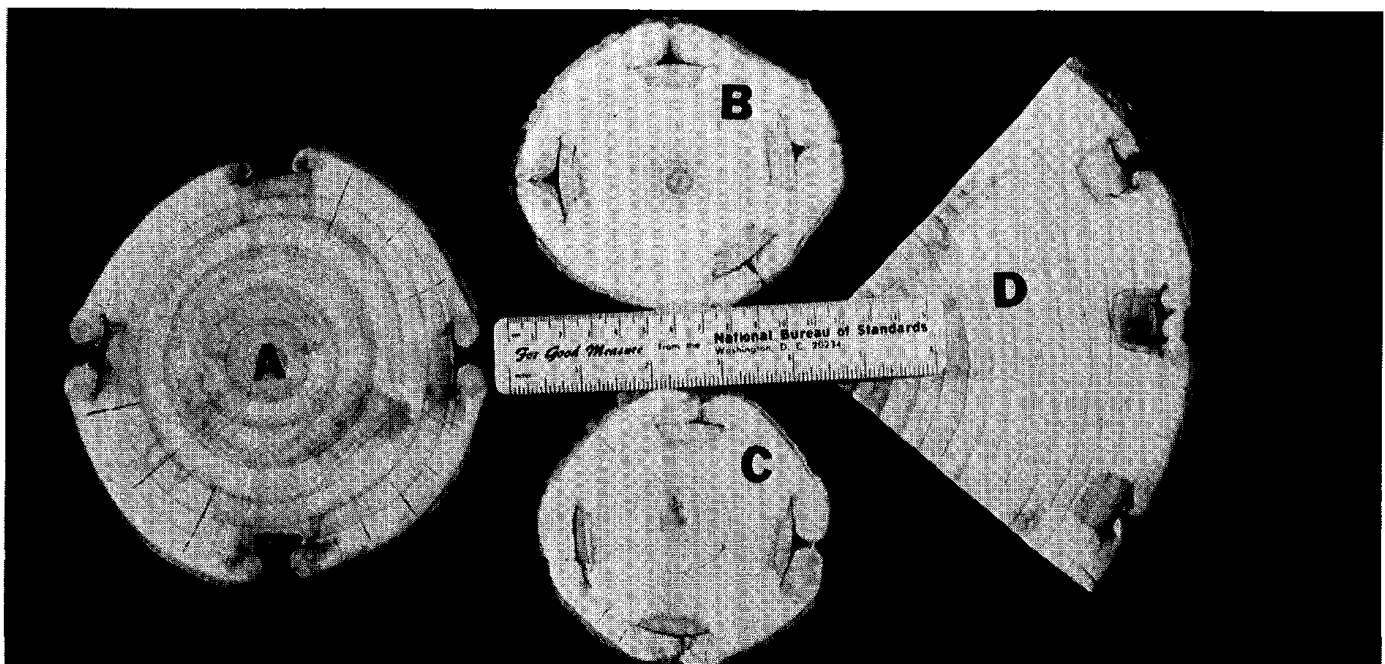
Fig. 2. Cross-sections of chisel-wounded trunks of hybrid poplars: (A) Clone NE-41 ('Androscoggin'), a weak compartmentalizer; (B) Clone NE-211, a strong compartmentalizer; (C) Clone NE-208, a weak compartmentalizer; (D) a strong compartmentalizing clone of unknown parentage. Note formation of Wall 2 between annual rings.
