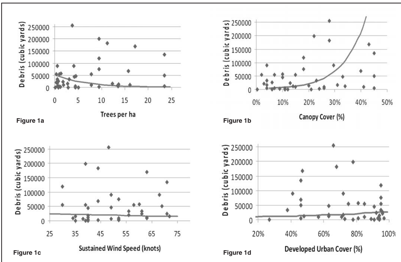
Figure 1. Predicted debris (cubic yards) versus (a) tree density (trees/hectare), (b) tree canopy cover (%), (c) sustained wind speed (kt), and (d) developed urban cover (%). Diamonds = raw data; solid line = predicted at constant average of all other predictor variables.
