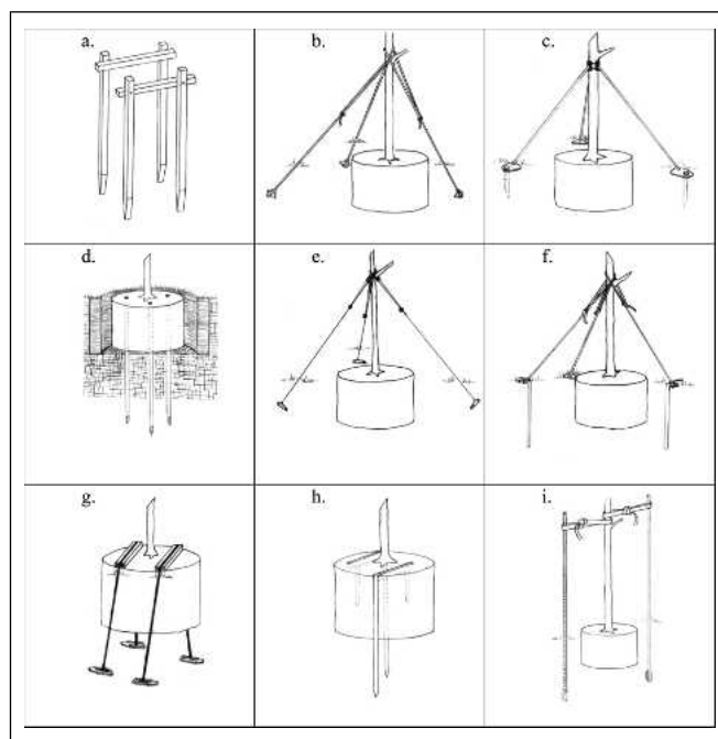
Figure 2. Illustrations of (A) 2 × 2's, (B) ArborBrace®, (C) Brooks Tree Brace®, (D) dowels, (E) Duckbill®, (F) rebar and ArborTie®, (G) Terra Toggle™, (H) Tree Staple™, and (I) T-stakes.
