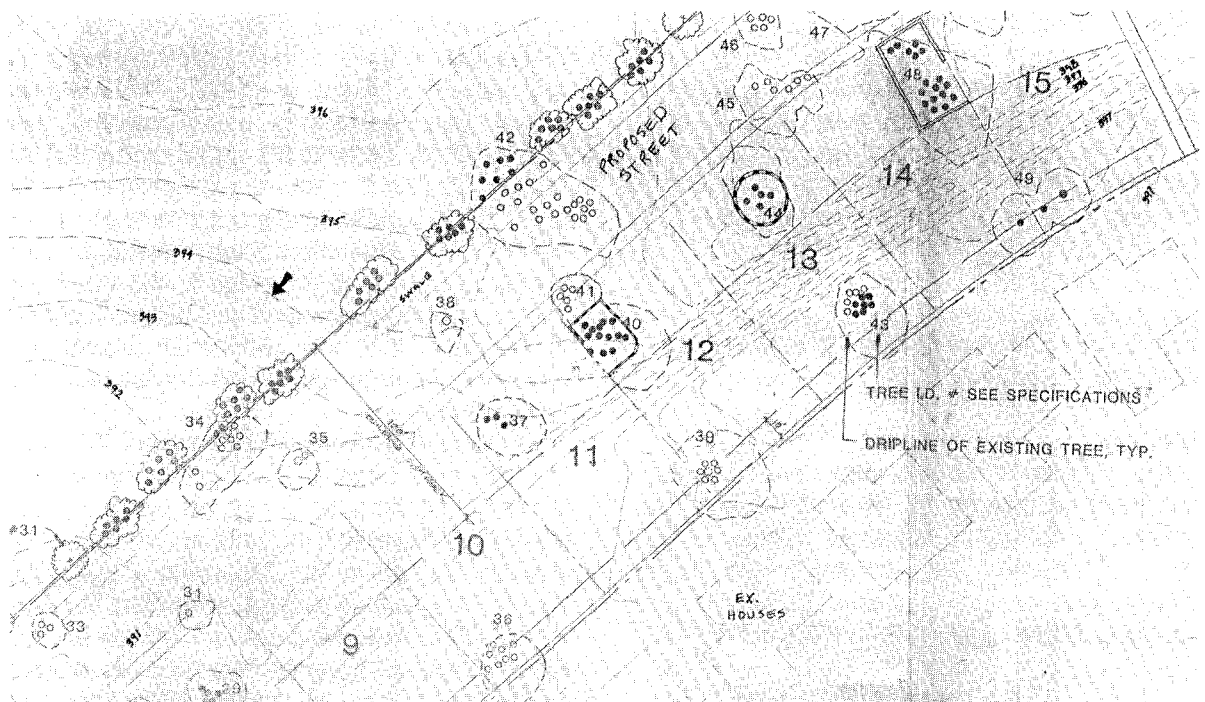
Figure 4. A portion of a plan for a subdivision. Proposed street location and parcel lot lines are shown. Note existing grade lines (small arrow), existing trees to remain (dark dots), and trees to be removed (white dots). Trees #40 and 44 show retaining walls proposed within the dripline. No new grade lines are shown. For this plan, the arborist must learn the elevations of the building pads for each lot and compare that to the existing grades shown.
